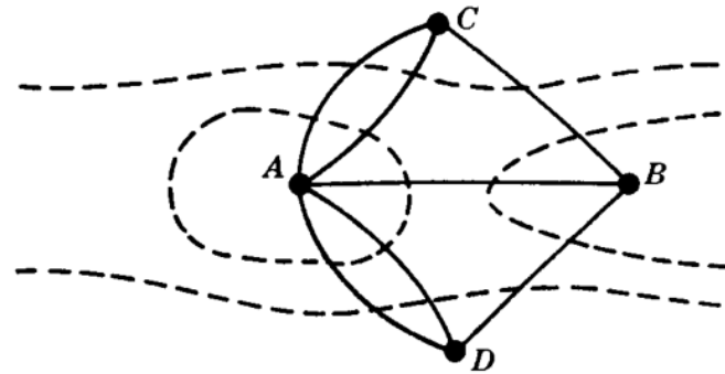
(b) Euler's graphical representation
